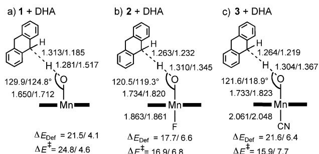
Figure 5. Key geometric details of 1 TS H / 3 TS H,B in 1–3 . Given underneath the TSs are the deformation energies (in kcal mol -1 ) of the species and the corresponding electronic barriers (UB3LYP/B2 + solv//B1 in kcal mol -1 ) relative to the separate reactants at a given spin state.
