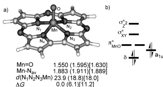
Figure 1. a) B3LYP key geometrical parameters (distances in Å, angles in °) and relative free energies (in kcal mol -1 ) for 1 , given in the order S=0 ( S_A=1 )[ S_B=1 ]. b) Orbital occupancy diagram for the S=0 state. S_A=1 has \delta^2\pi^*a_{1u}^1 while S_B=1 has \delta^1\pi^*a_{1u}^2 .
